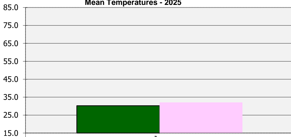
Mean Temperatures - 2025
