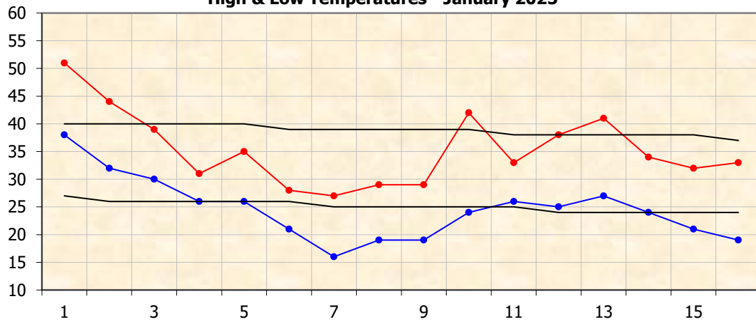
High & Low Temperatures - January 2025
