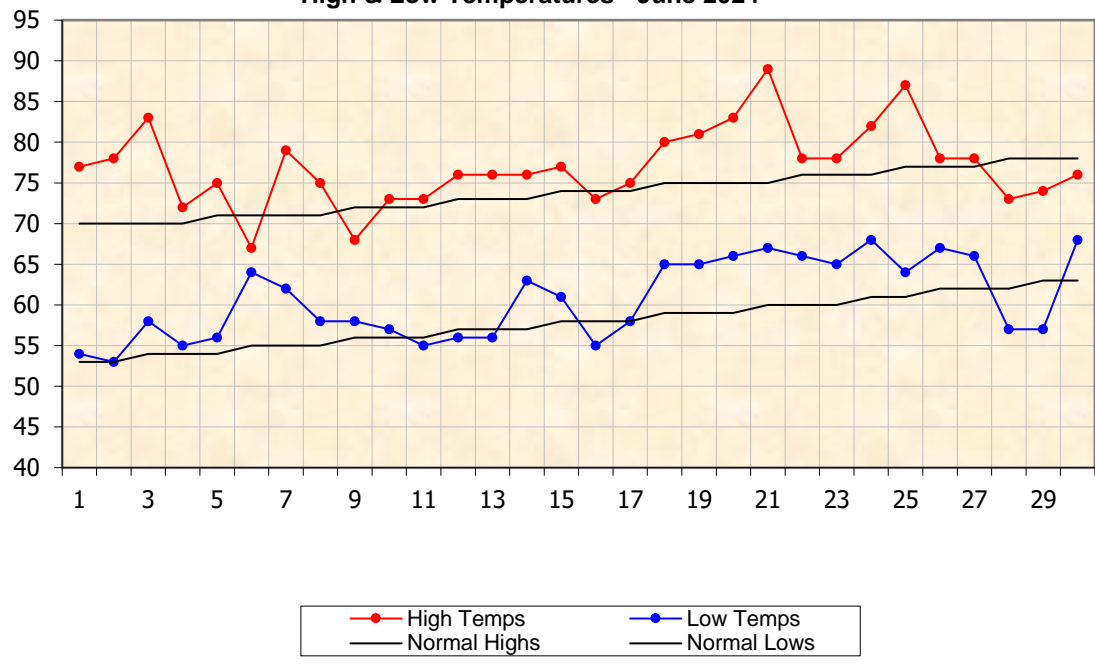
High & Low Temperatures - June 2024
